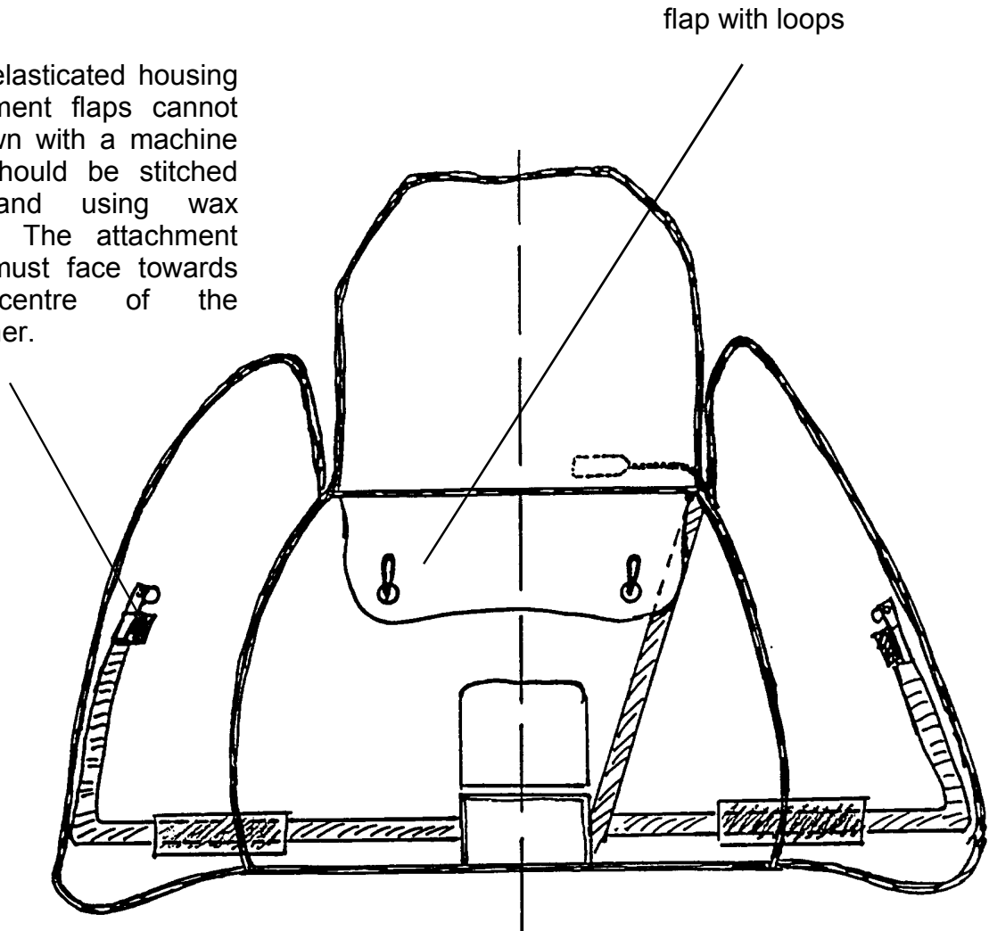
unit cable housing routed underneath the velcro strips
